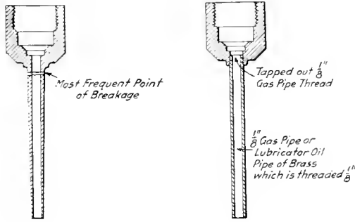
Method of Making Emergency Repairs to an Injector Priming Nozzle
